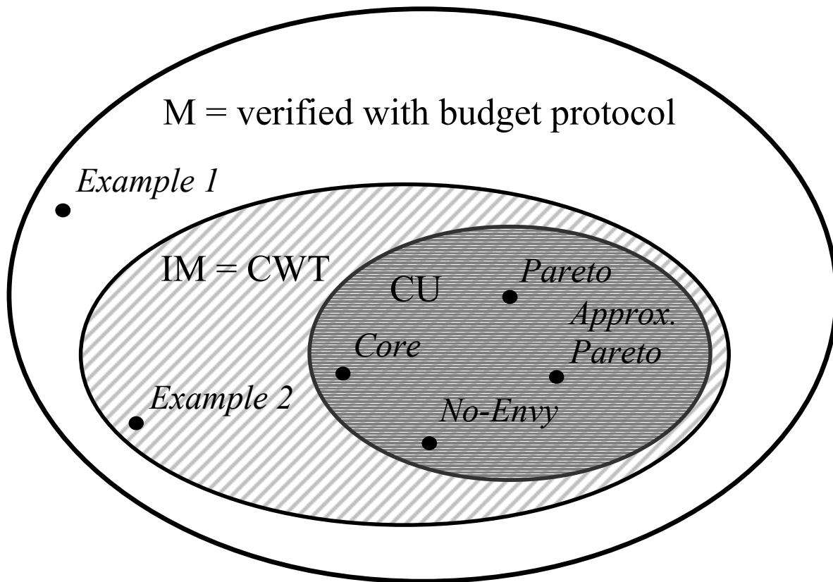
Figure 4: Venn Diagram for Choice Rules
